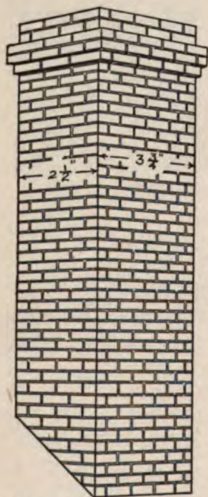
FIG. 227. — The Chimney.
